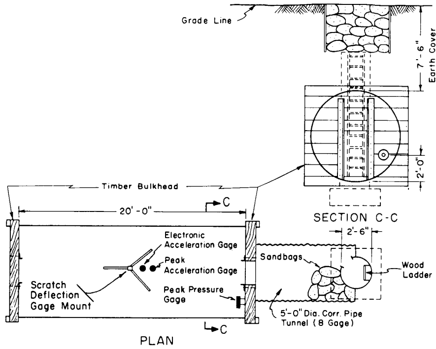
Fig. 8—Typical gauge locations inside test section.
